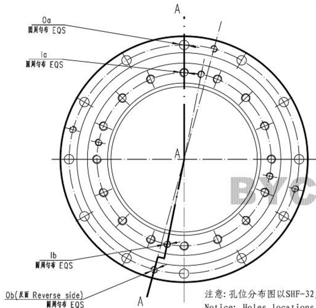
交叉滚子轴承配套用于SHF/SHG型谐波减速机 (Cross Roller Bearing used for SHF/SHG Harmonic Drive)
